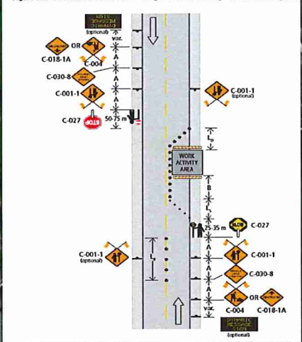
Figure 7.8: Lane Closure with TCPs – Single Lane Alternating – Short and Long Dur
